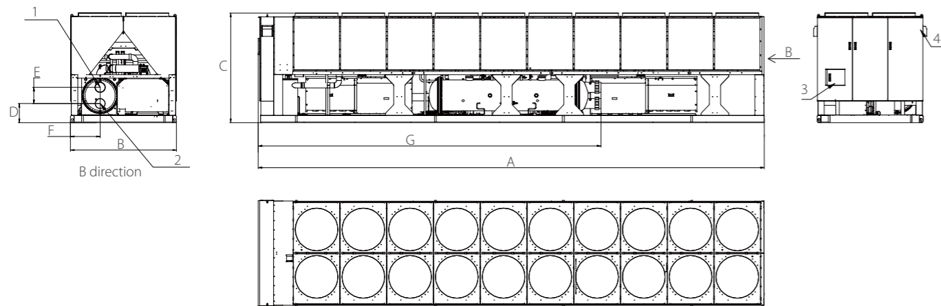
① Chilled water outlet ② Chilled water inlet ③ Control panel ④ Power incoming line
