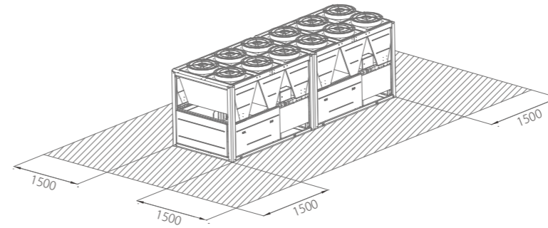
Series connection
