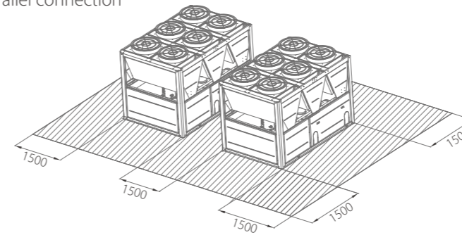
Parallel connection
