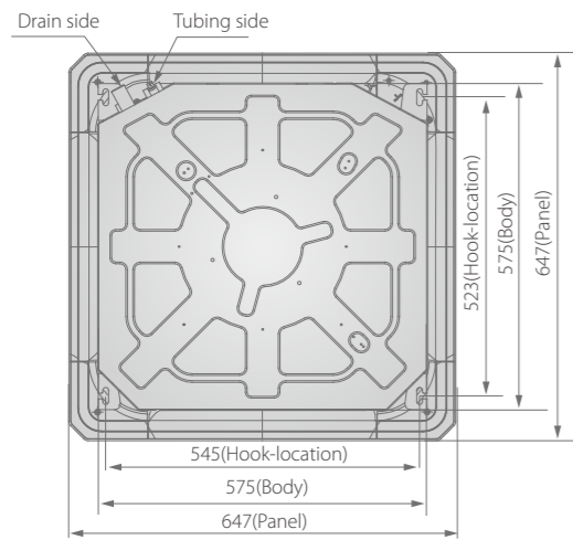
4-pipe compact 4-way cassette Dimensions (unit: mm)
