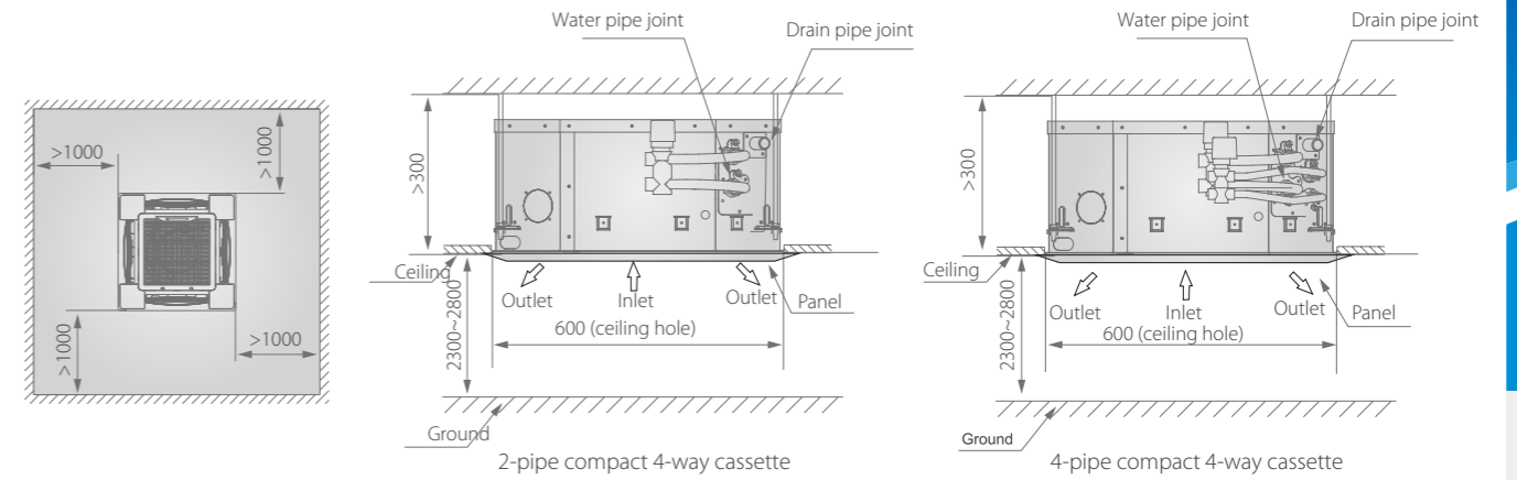
Service Spaces (unit: mm)
