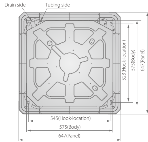
2-pipe compact 4-way cassette Dimensions (unit: mm)
